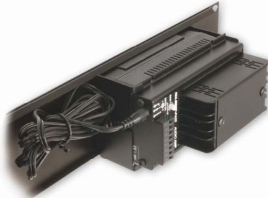
FP-PSB1 mounted in FP-RRR (with PS-24U2 supply and FP-PA20 amplifier)
